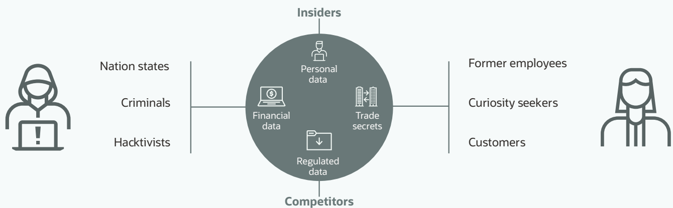
Figure 1.2: Threat actors
