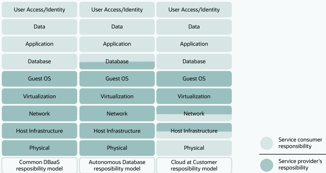
Figure 12.3: DBaaS shared responsibility model
