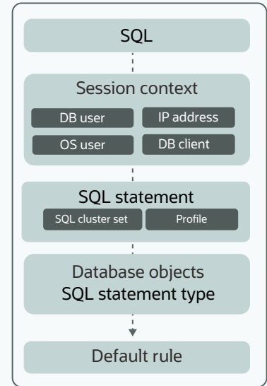
Figure 8.3: Multi-stage Database Firewall
