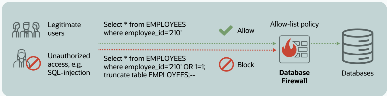
Figure 7.3: Monitoring network traffic with Database Firewall
