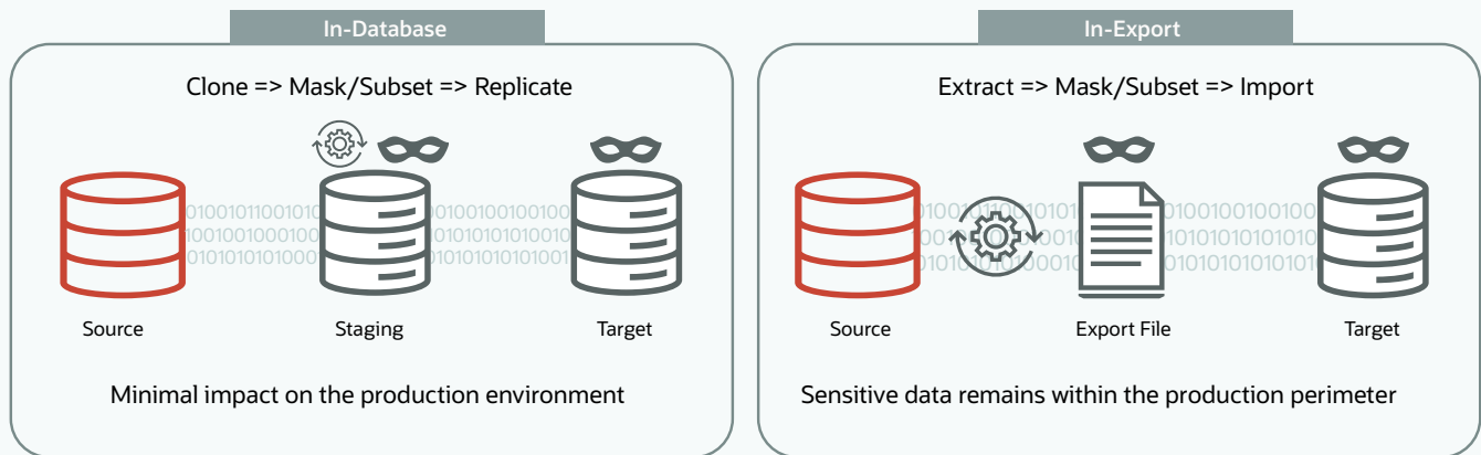
Figure 6.6: Data masking and subsetting modes
