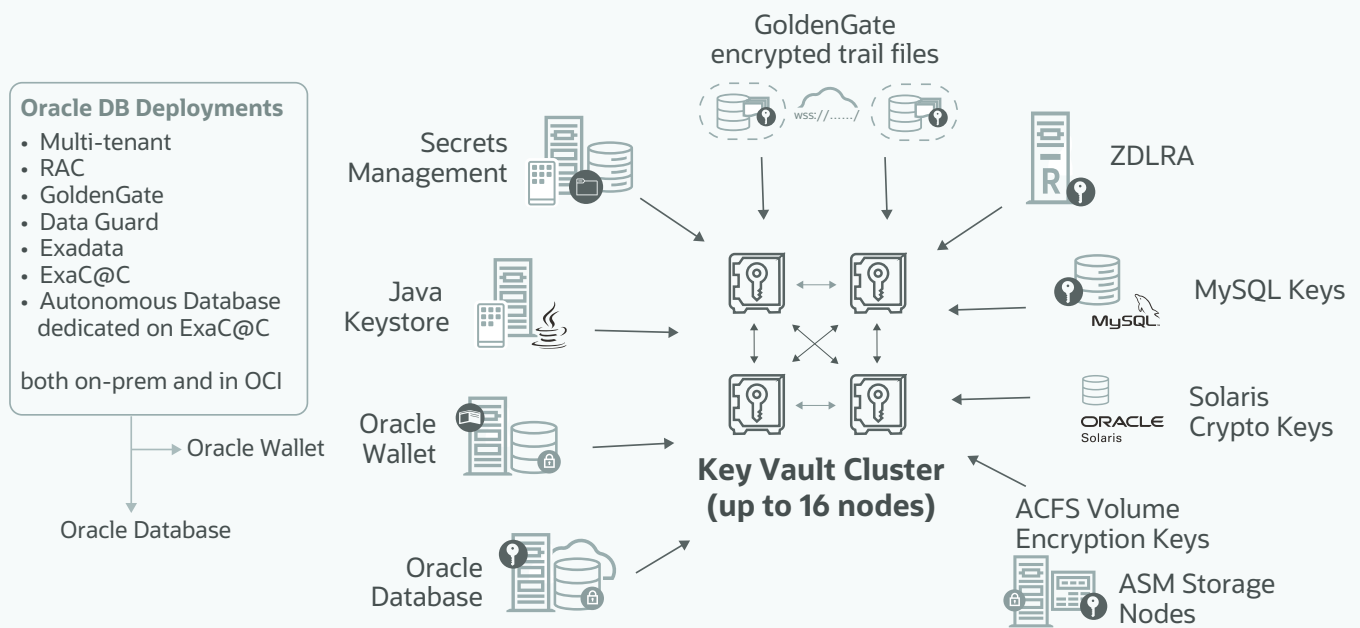
Figure 4.4: Oracle Key Vault manages Oracle TDE MEKs, as well as other keys and security objects.
