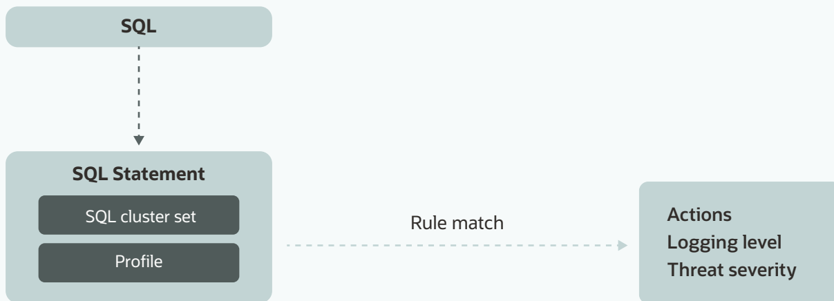
Figure 8.5: SQL statement rules
